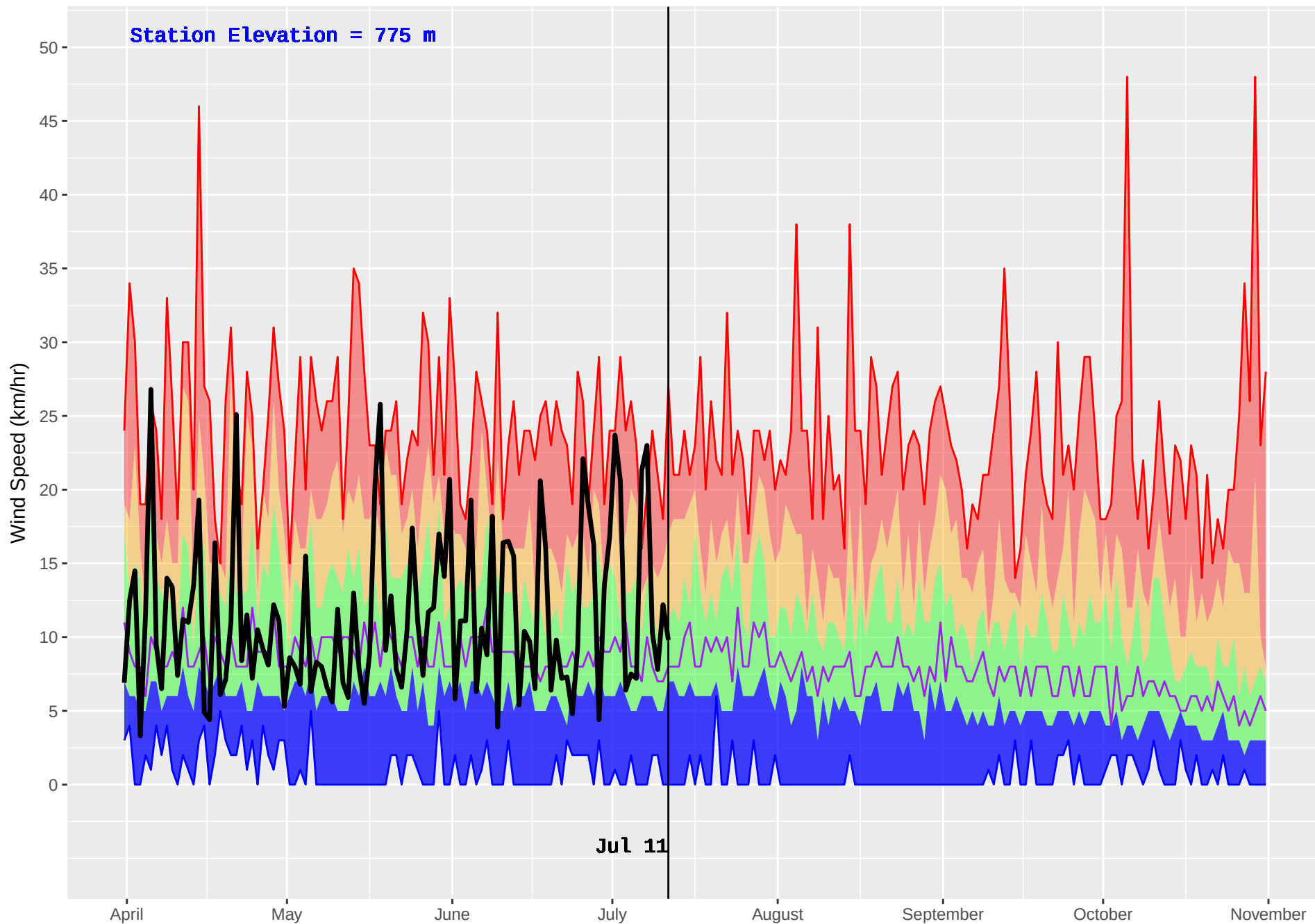
ELKO (412) : Historical (1970–2016) and Current (2018) Noon Wind Speed
