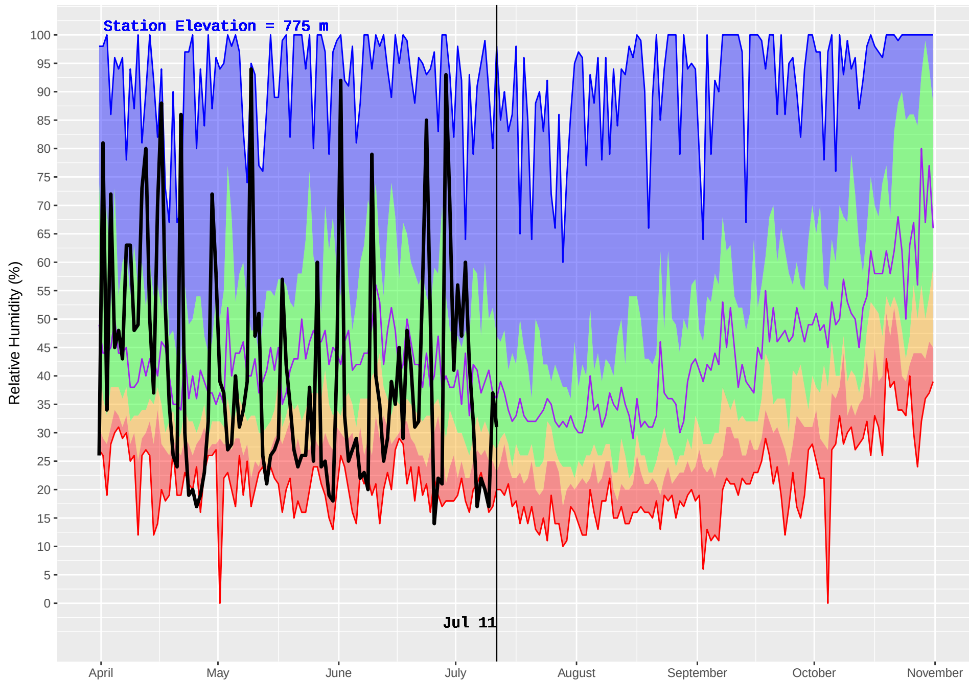
ELKO (412) : Historical (1970–2016) and Current (2018) Noon Relative Humidity
