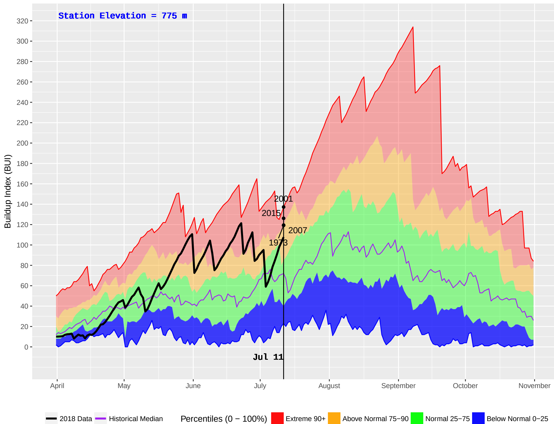
ELKO (412) : Historical (1970–2016) and Current (2018) Noon Buildup Index (BUI)
