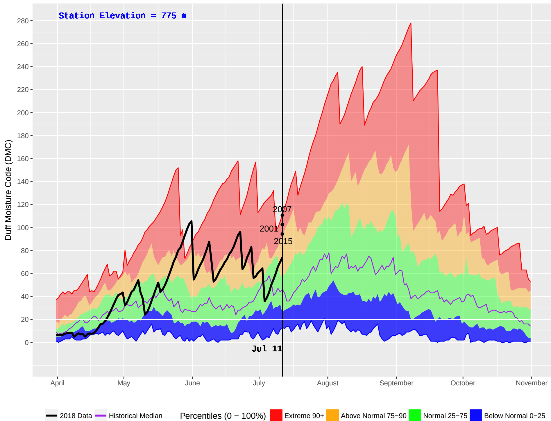
ELKO (412) : Historical (1970–2016) and Current (2018) Noon Duff Moisture Code (DMC)
