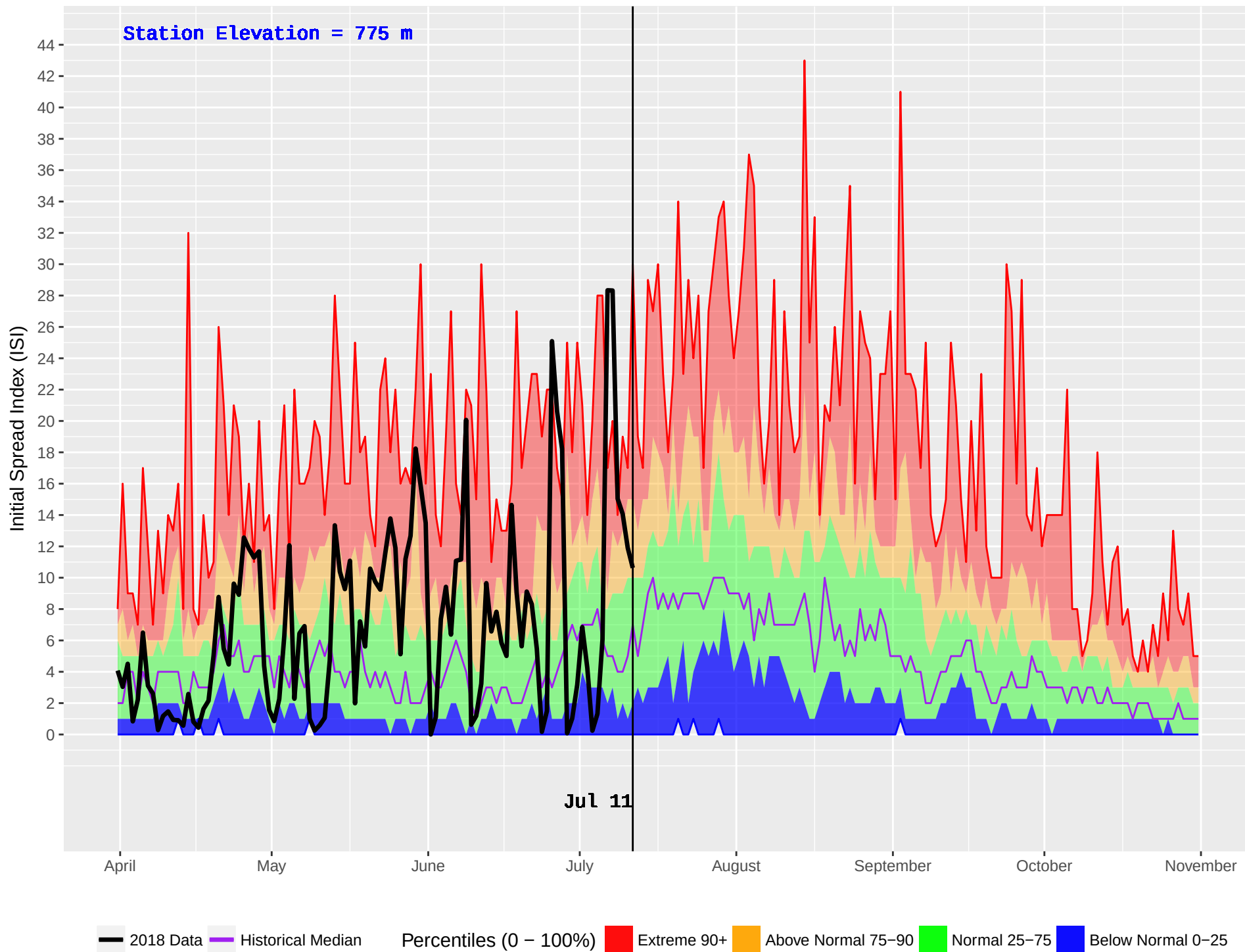
ELKO (412) : Historical (1970–2016) and Current (2018) Noon Initial Spread Index (ISI)
