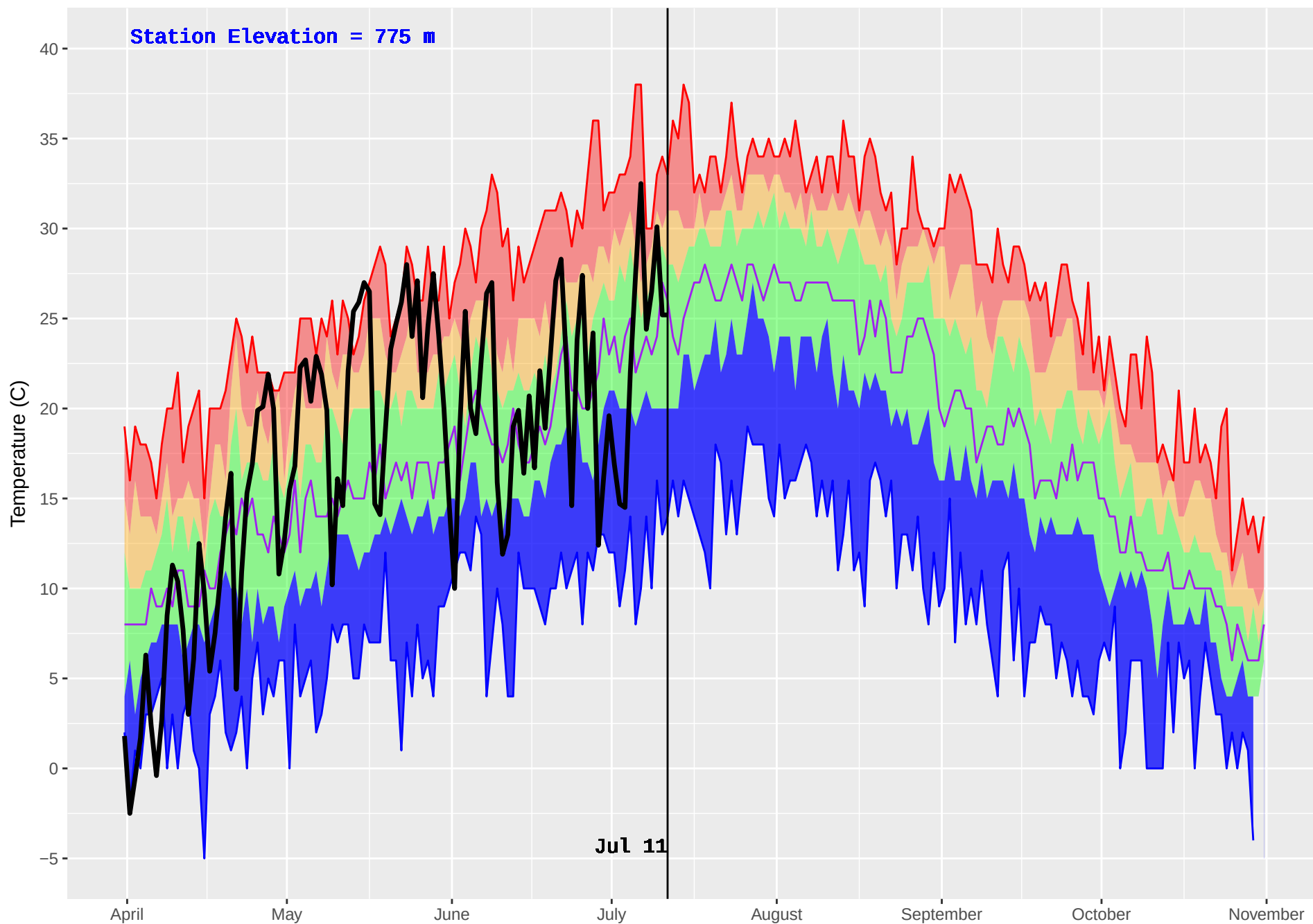
ELKO (412) : Historical (1970–2016) and Current (2018) Noon Temperature
