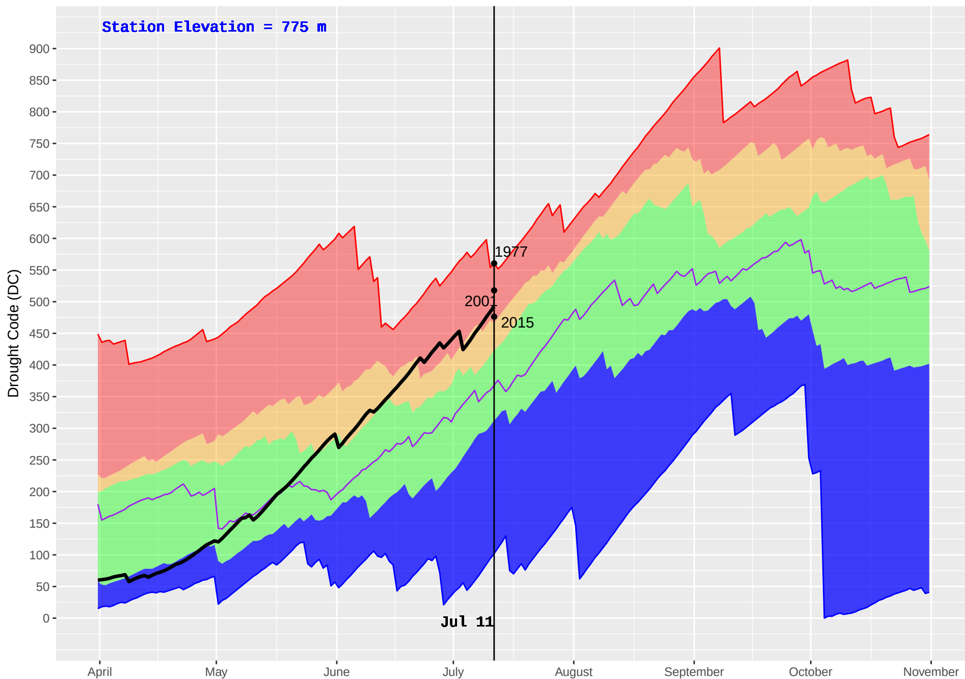
ELKO (412) : Historical (1970–2016) and Current (2018) Noon Drought Code (DC)
